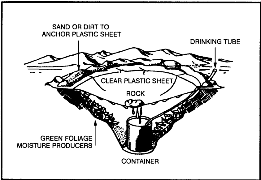
Figure 6-7. Belowground still.
