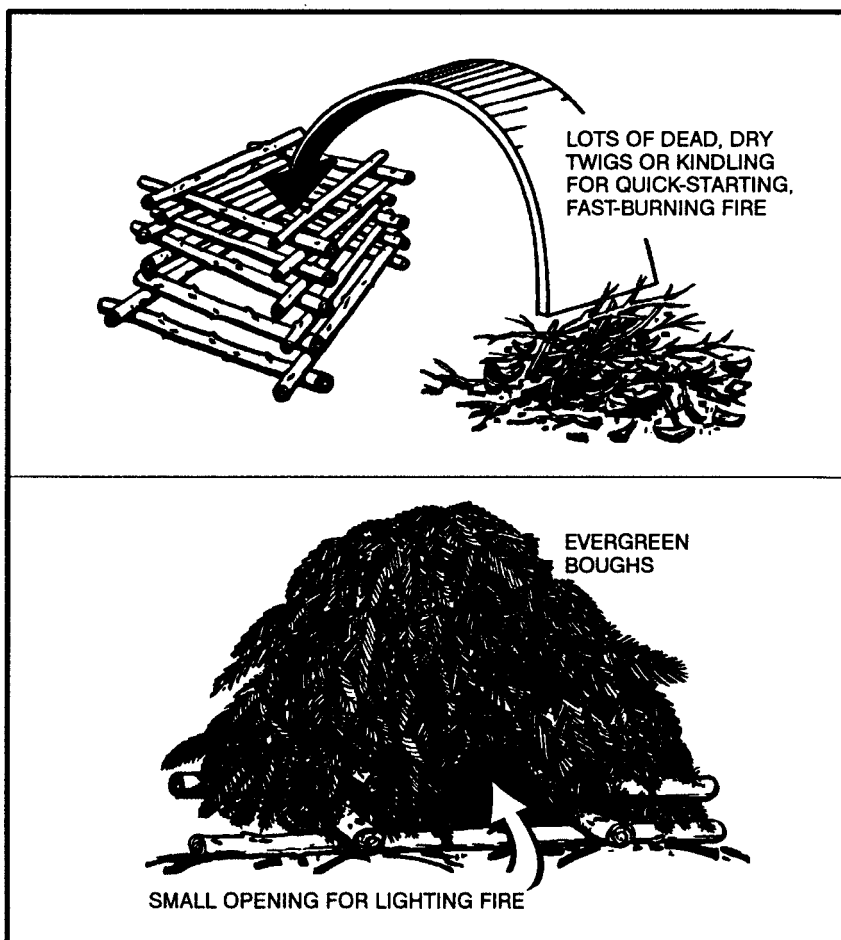
Figure 19-2. Smoke generator—ground.
