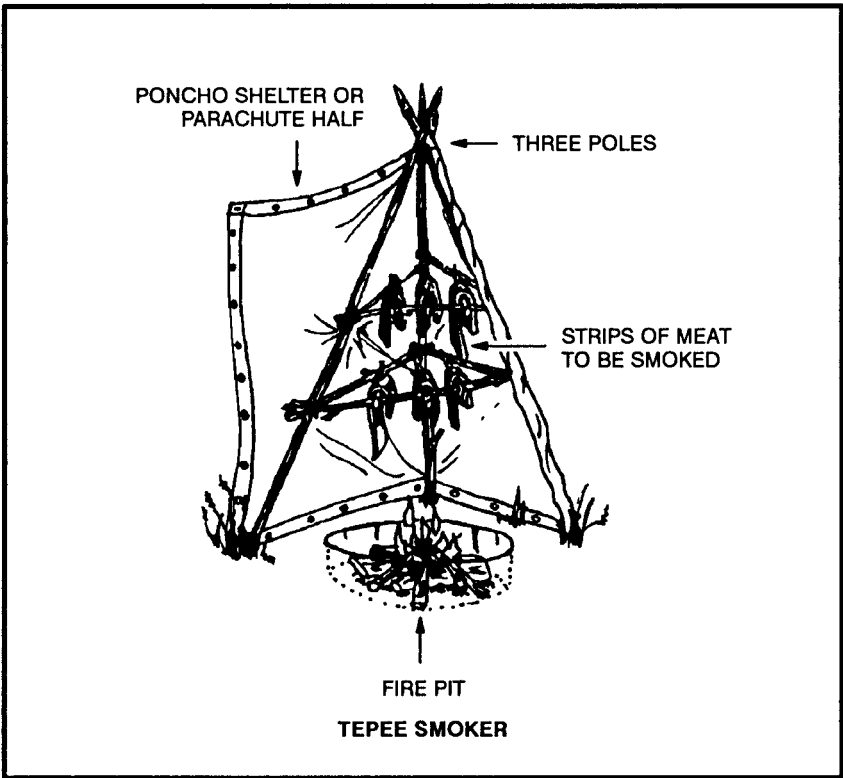
Figure 8-27. Smoking meat.
