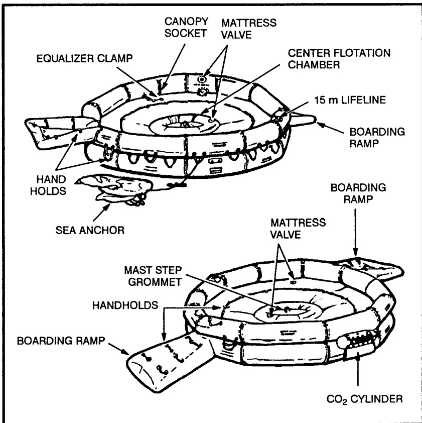
Figure 16-15. Twenty-man raft.
