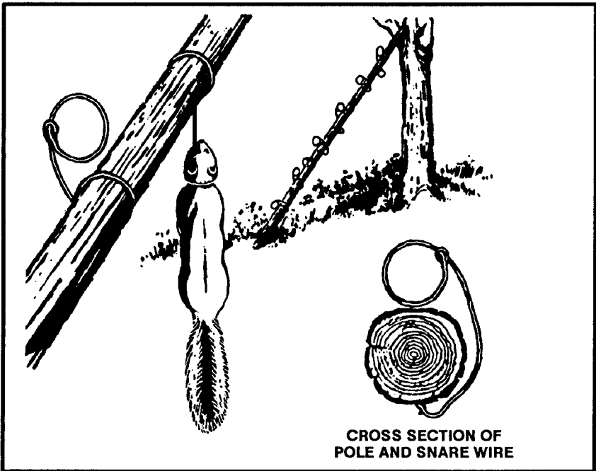
Figure 8-7. Squirrel pole.
