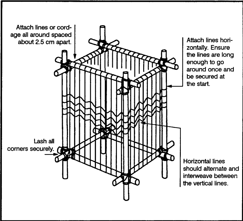
Figure 12-10. Square pack.
