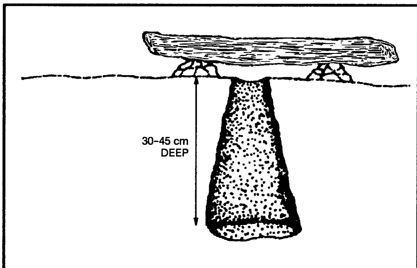
Figure 8-16. Bottle trap.
