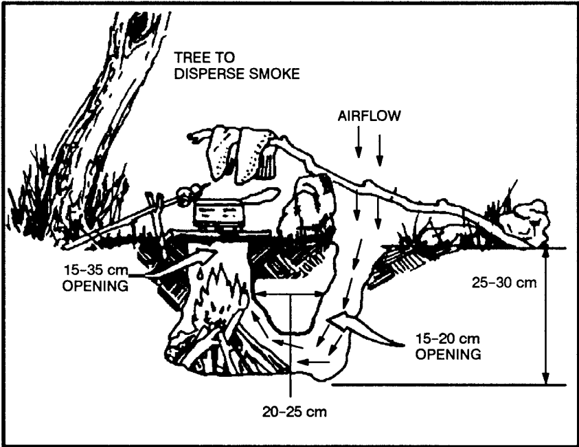
Figure 7-2. Dakota fire hole
