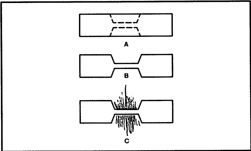
Figure 4-7. Butterfly closure.
