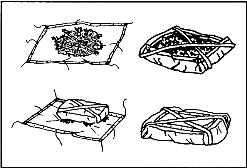
Figure 17-4. Brush raft.
