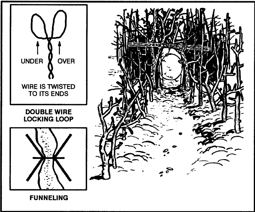
Figure 8-6. Drag noose.
