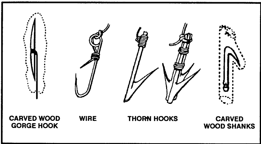
Figure 8-17. Improvised fishhooks.
