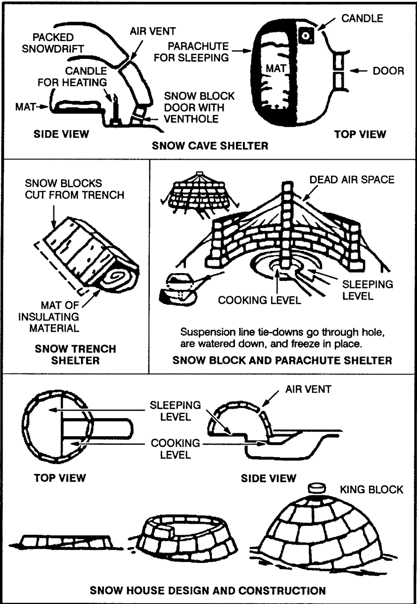
Figure 15-4. Snow houses.
