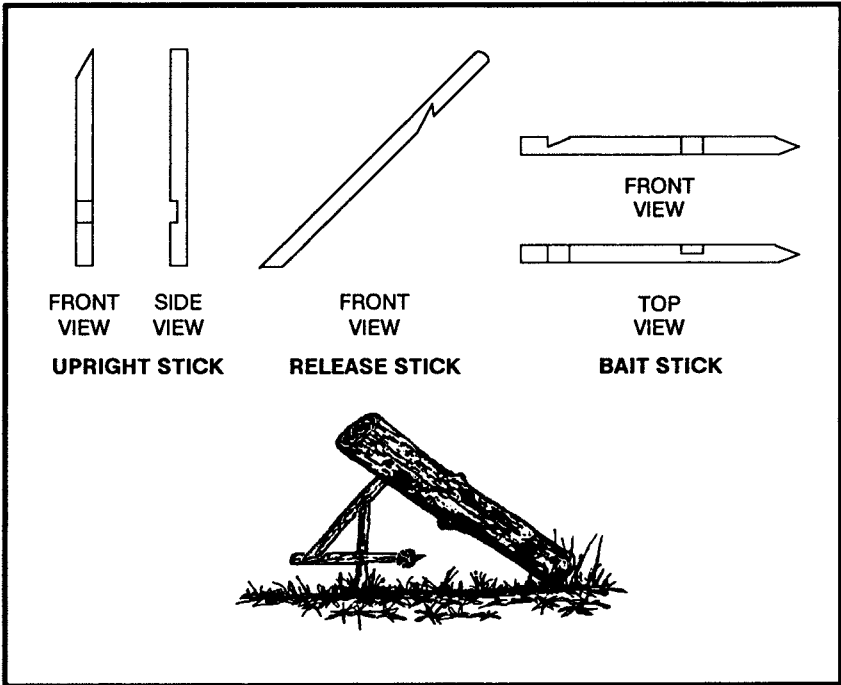
Figure 8-11. Figure 4 deadfall.
