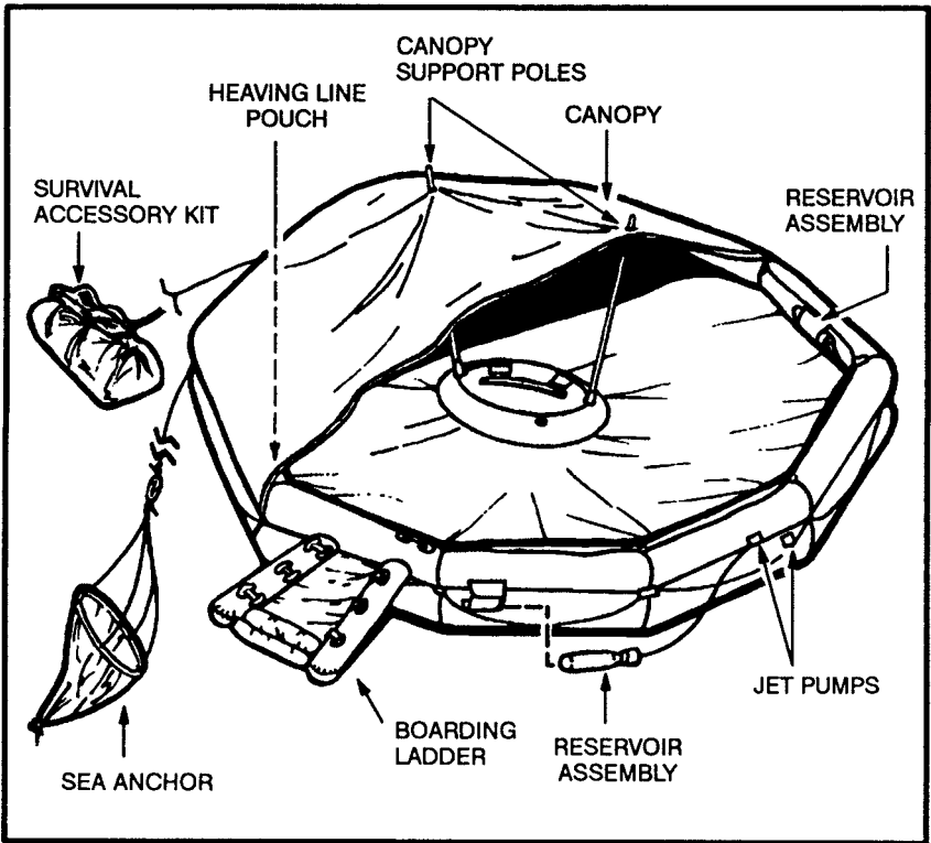
Figure 16-16. Twenty-five-man raft.
