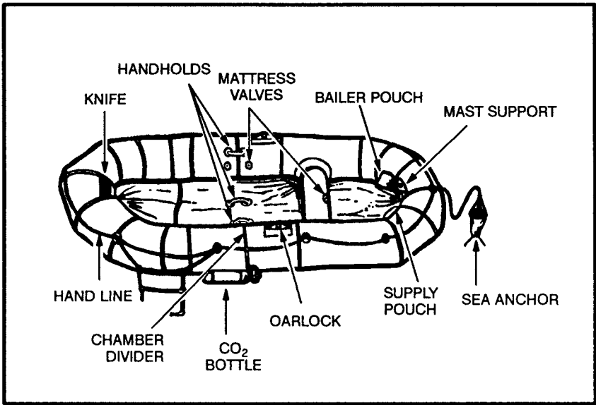
Figure 16-12. Seven-man raft.
