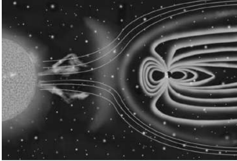
Figure 51: Planetary magnetospheres are formed by an electrical charge within plasma meeting another electrical charge which causes a barrier to be formed.
