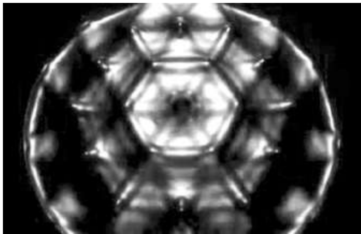
Figure 131: A sound pounding through a liquid medium creates a perfect hexagon.
