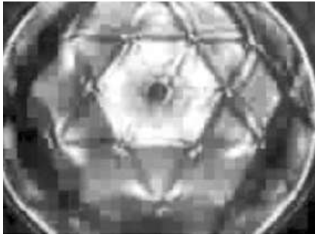
Figure 130: Sound impacts on the medium to form a hexagram or Star of David/Seal of Solomon..
