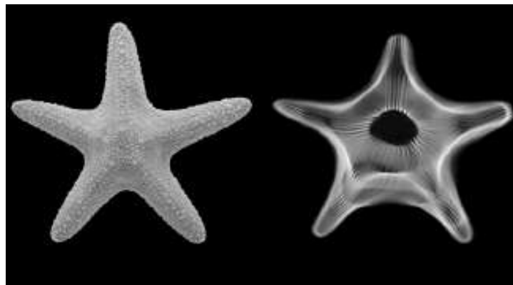
Figure 25: A real starfish and a 'starfish' created by cymatics.
