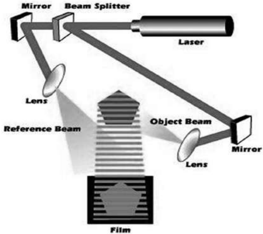
Figure 38: Two parts of a laser collide on the holographic print to form a wave pattern.
