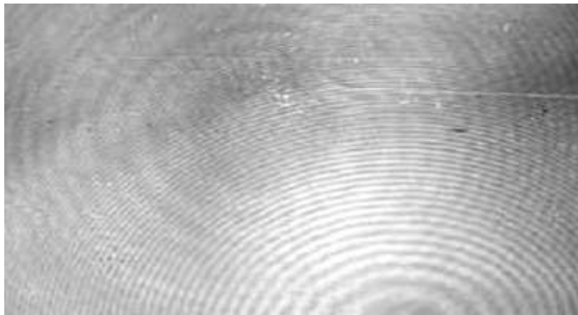
Figure 39: Holographic prints are created from the interaction of waves and are encoded with the information of the object being holographically photographed.
