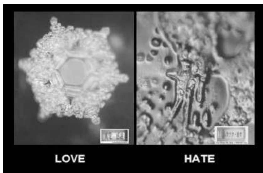
Figure 81: Water crystals infused with the vibration from words of love and hate. No difference, then?
