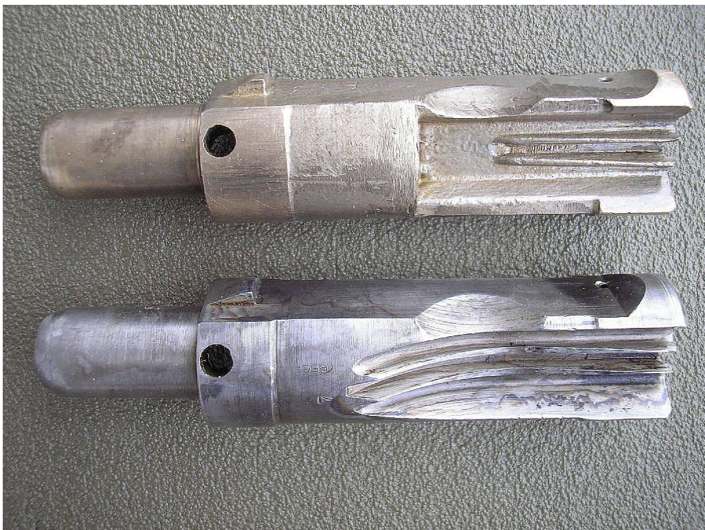
Top: cast bronze, bottom: machined steel:
