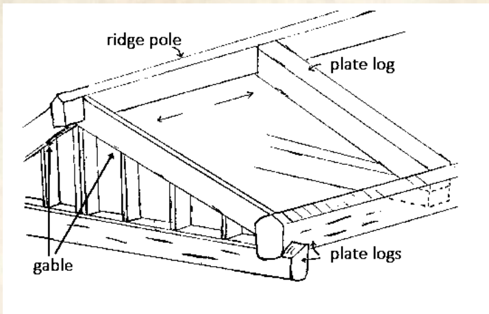
Figure 32. Roof truss: gable, ridge pole & plate logs
