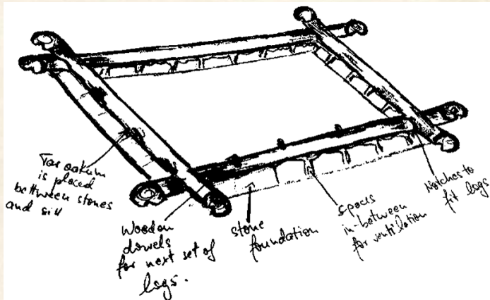
Figure 21. Stone foundation & sill
