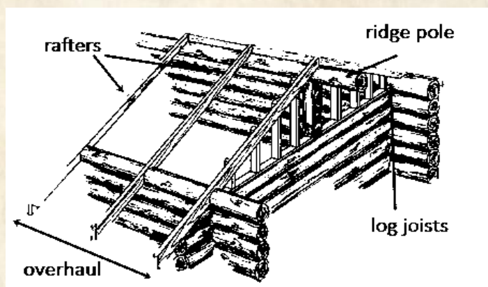
Figure 33. Cabin roof joists & overhaul
