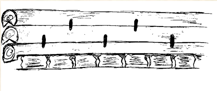
Figure 23. Dowels in between logs for stability
