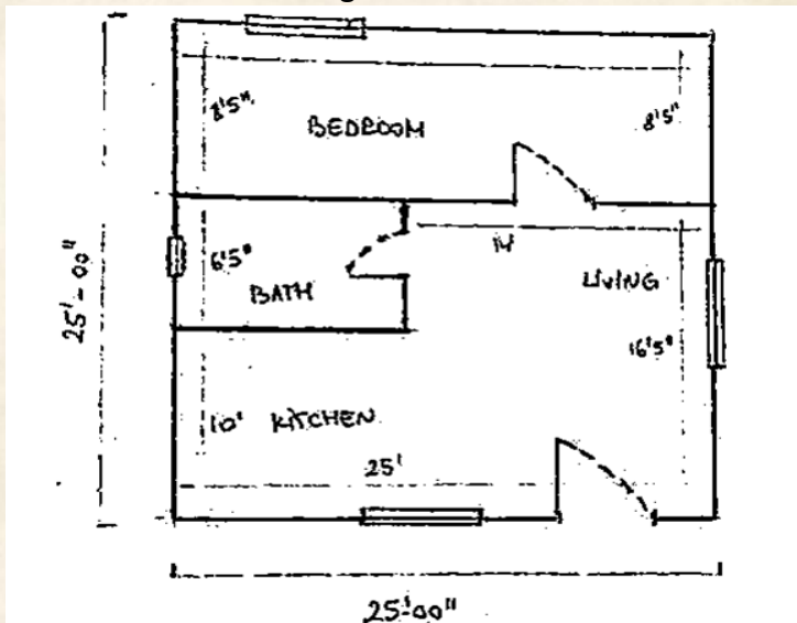
Figure 12. Log cabin
