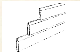
Figure 30. Shiplapping ceiling planks
