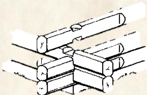
Figure 19. Lock notching
