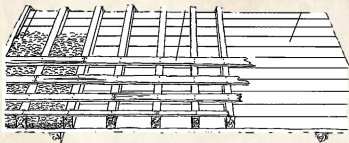
Figure 26. Dirt flooring
