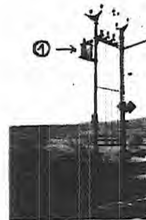
Destruction of main pole (usually across from station building) If you have little time: fire into the oil insulator (1). If you have sufficient time: blast the pole at place (2) indicated by arrow.
